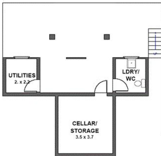
LOWER LEVEL
