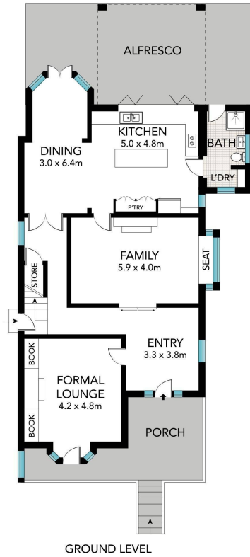
GROUND LEVEL
